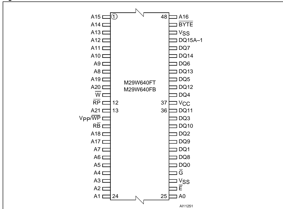
Figure 2. TSOP Connections
